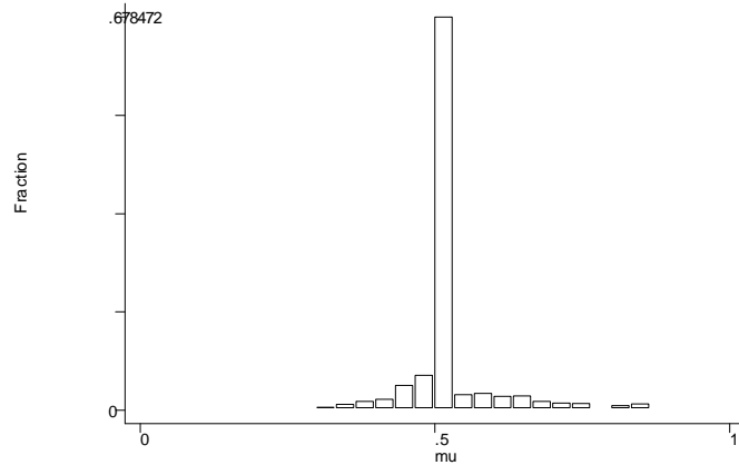
Figure 2: distribution of the power index
