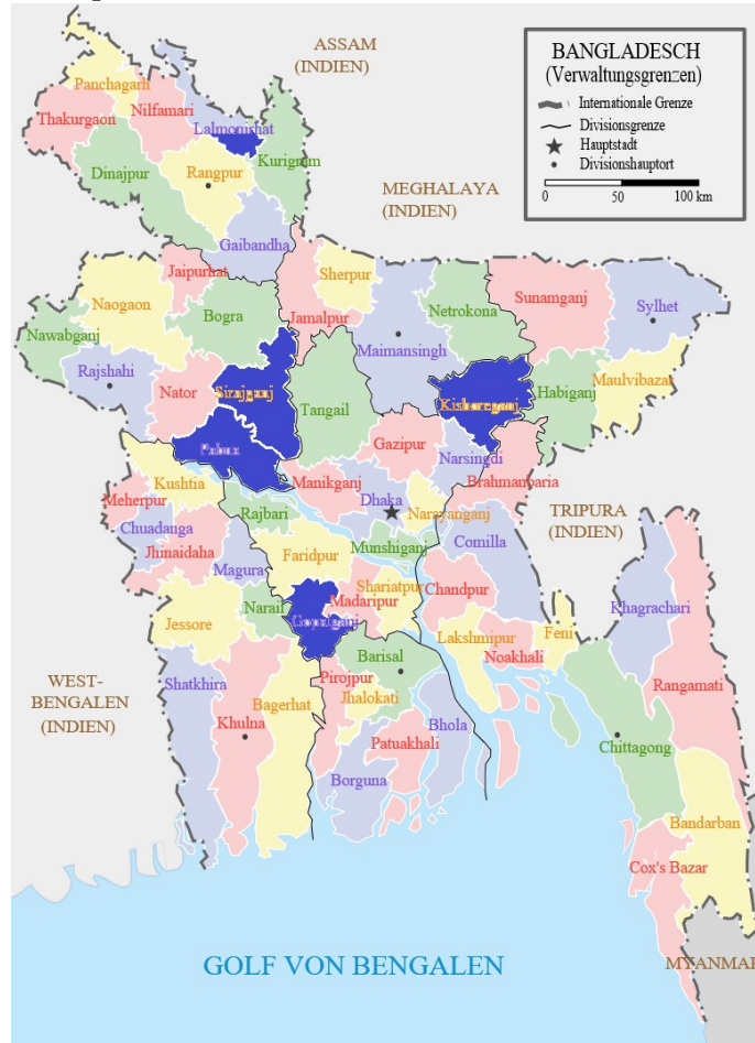
Figure B1: Districts in the field experiment
