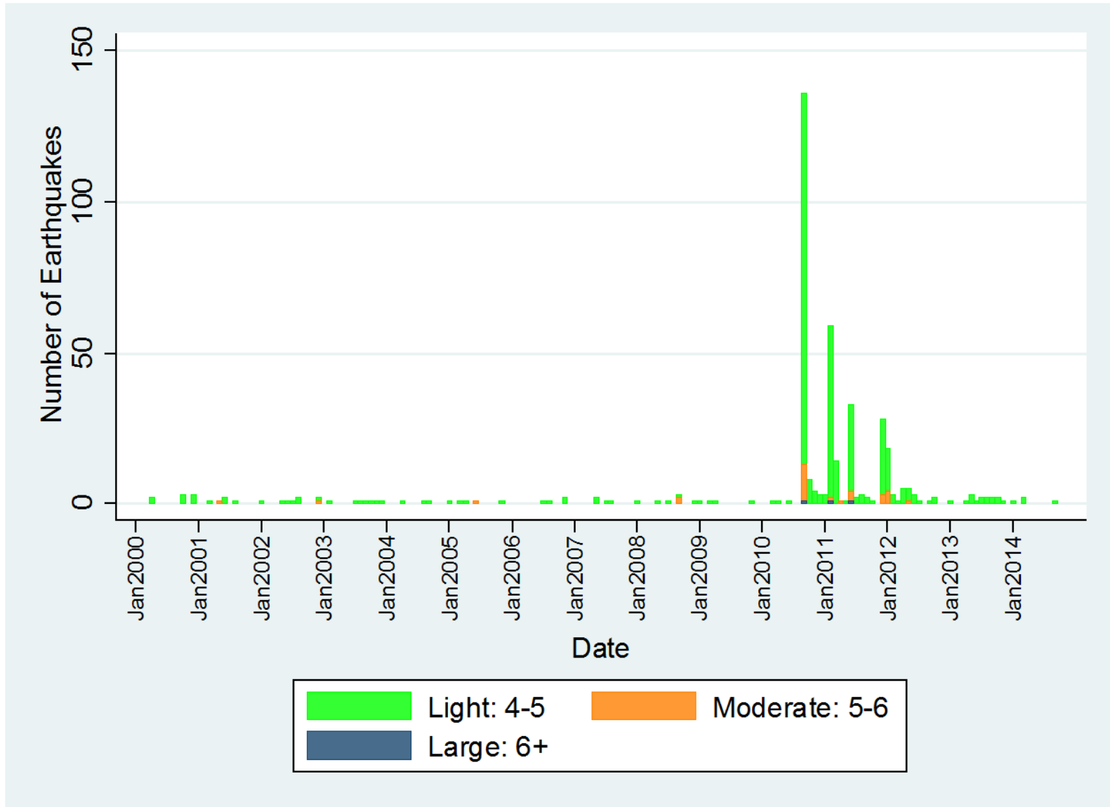
Figure 1. Earthquakes in the 'Affected Area' of Greater Christchurch; Years 2000-2014 (Monthly Number)
