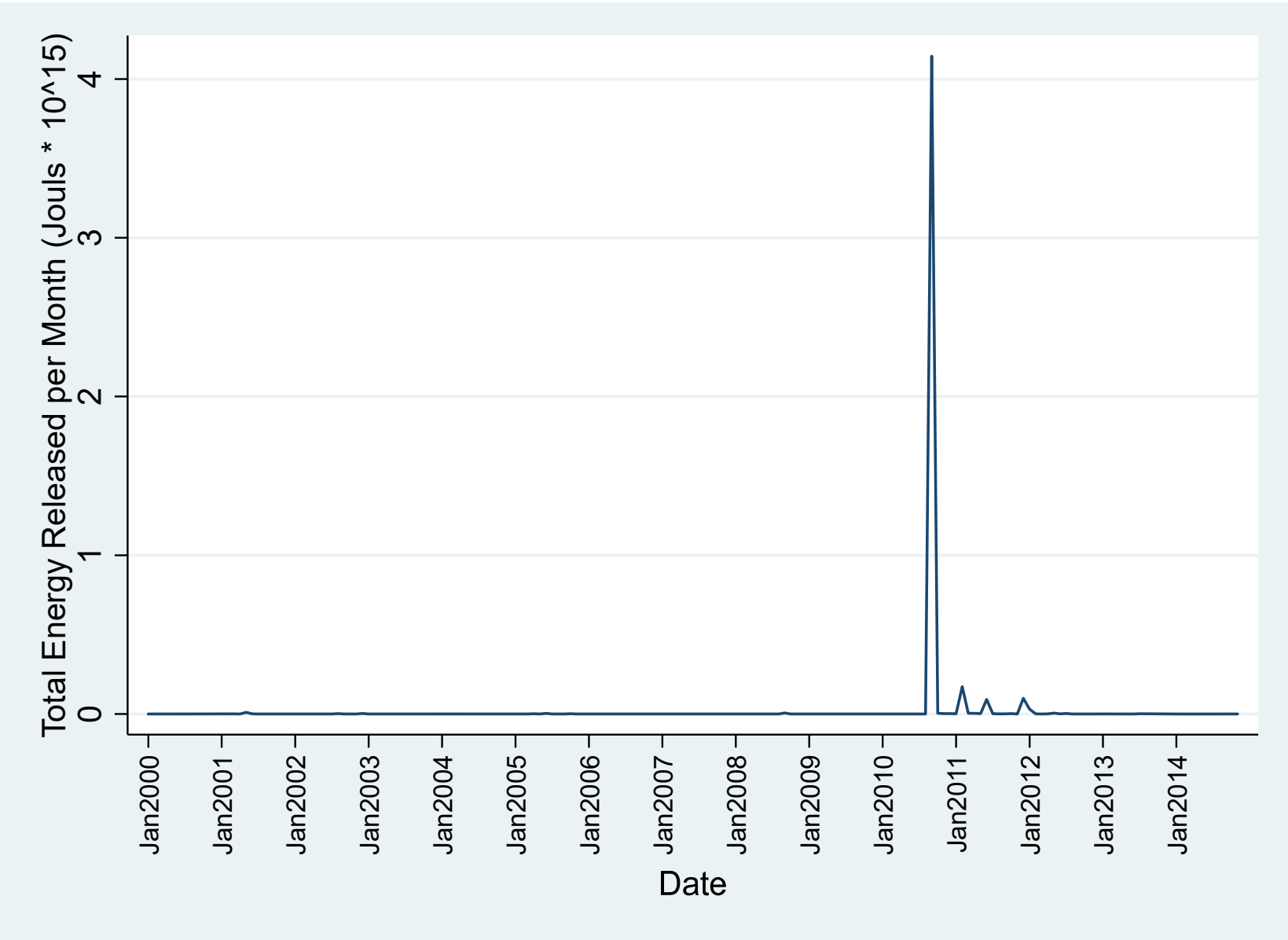
Figure 2. Earthquakes in the 'Affected Area' of Greater Christchurch; Years 2000-2014 (Monthly Energy Released)
