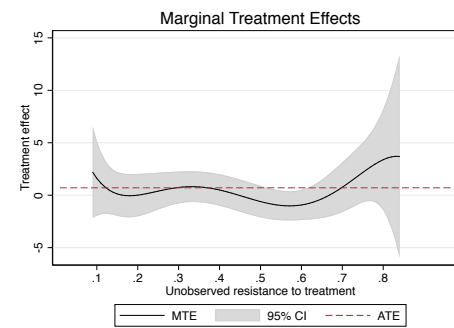
(f) Polynomial Degree 5
