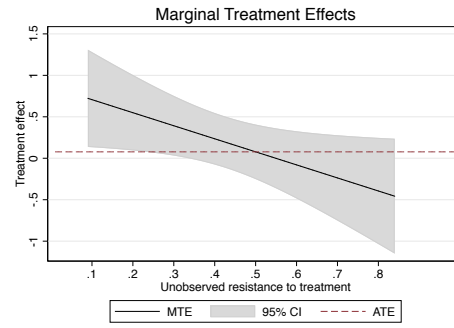
(b) Polynomial Degree 1
