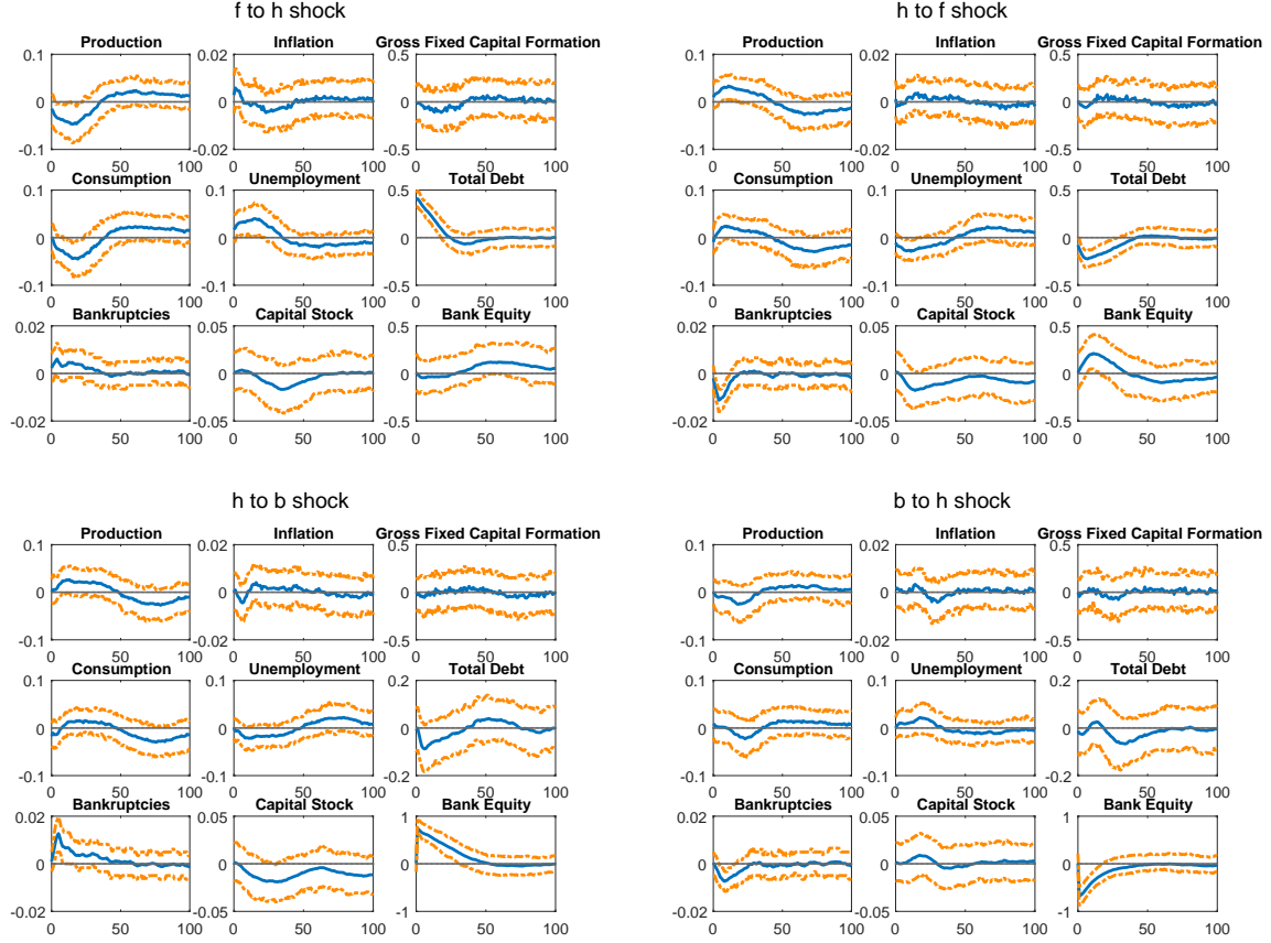
Figure 7: Upper left :RIRs of redistribution from firms to households. Upper right :RIRs of redistribution from households to firms. Lower left : RIRs of redistribution from household to the bank. Lower right : RIRs of redistribution from the bank to households. Period 0 corresponds to the period in which the shock hits the economy.
