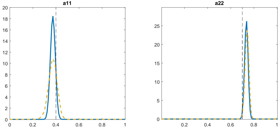
Figure 12: Posterior distribution of a_{11} and a_{22} using the Bayesian estimation including one lag in the likelihood (continuous blue line) and using the Bayesian estimation without lags. The vertical dashed lines represent the true value of the parameters.
