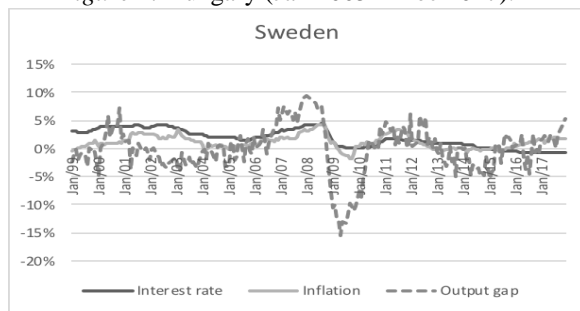
Figure 4. Sweden (Jan 1999 – Dec 2017).
