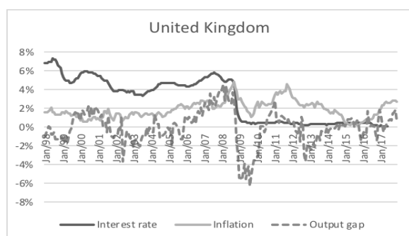
Figure 5. United Kingdom (Jan 1998 – Dec 2017).
