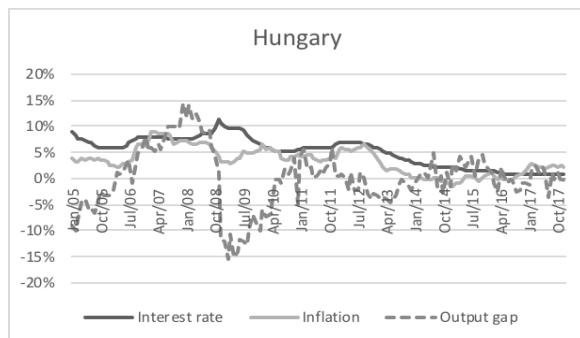
Figure 2. Hungary (Jan 2005 – Dec 2017).
