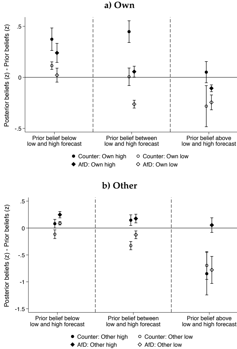
Figure 1: Belief updating
