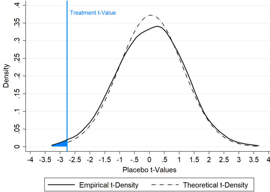
Figure 3: Randomized Rainfall
