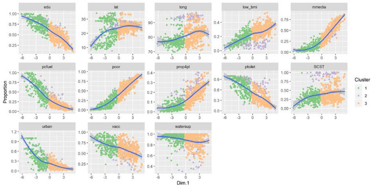
Figure 5. Various risk factors and principal component #1 for different clusters
