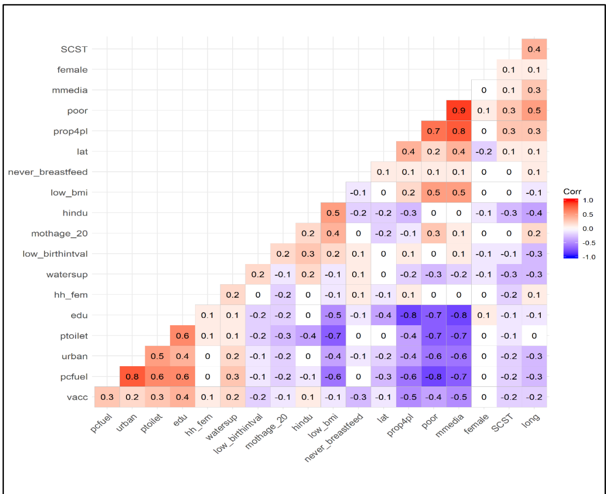
Figure 1. Correlogram for independent variables identified as relevant for explaining differences in average height and weight of children under the age of five
