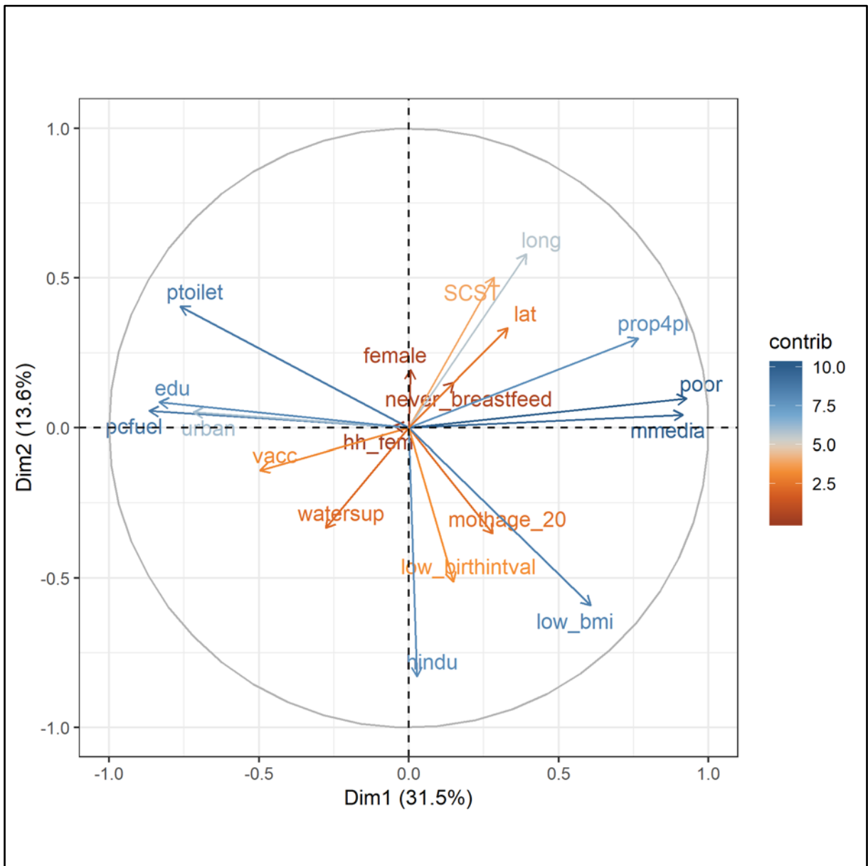
Figure 2. Contribution of different variables to first two principal components
