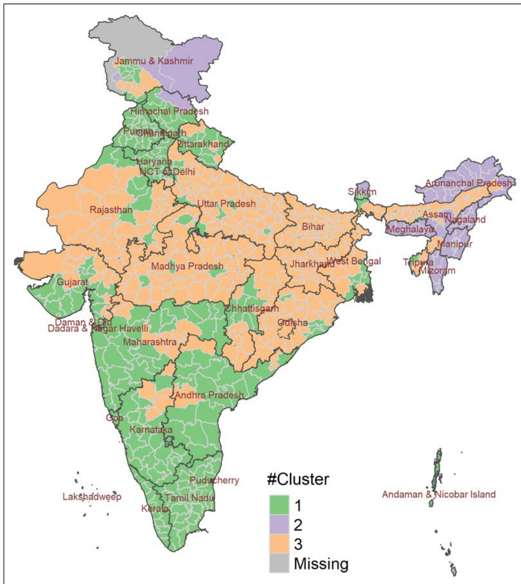
Figure 4. Clusters derived from principal components, India, 2016
