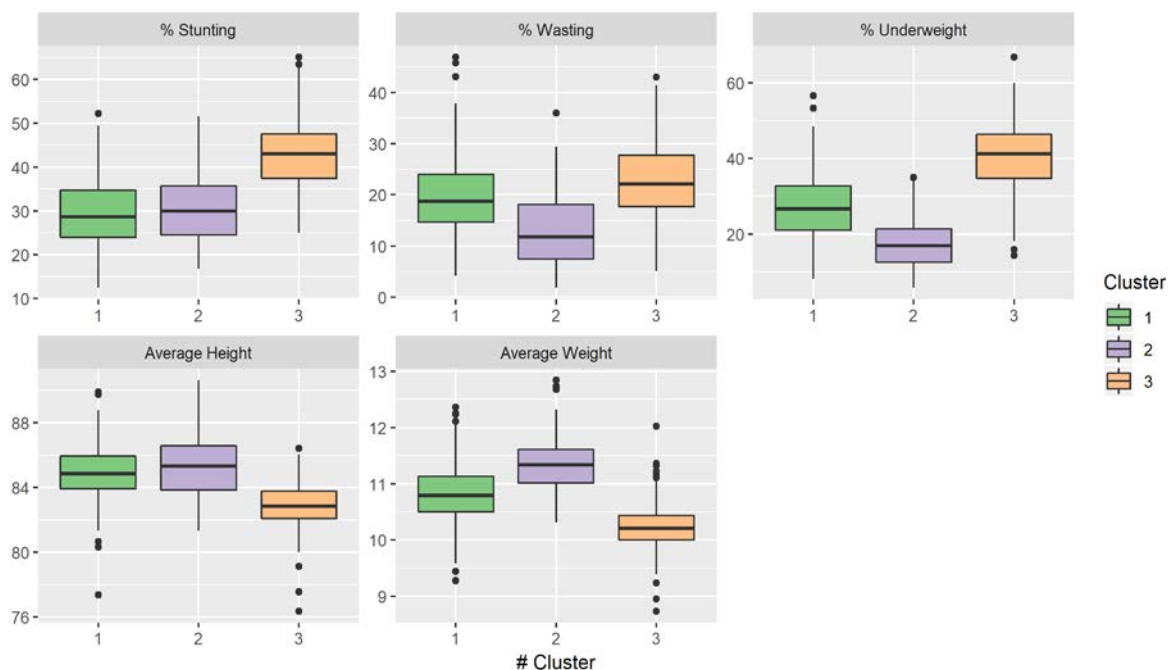
Figure 6. Distribution of wasting, stunting, underweight, as well as average height and weight across Indian districts for three different groups of counties identified by cluster analysis
