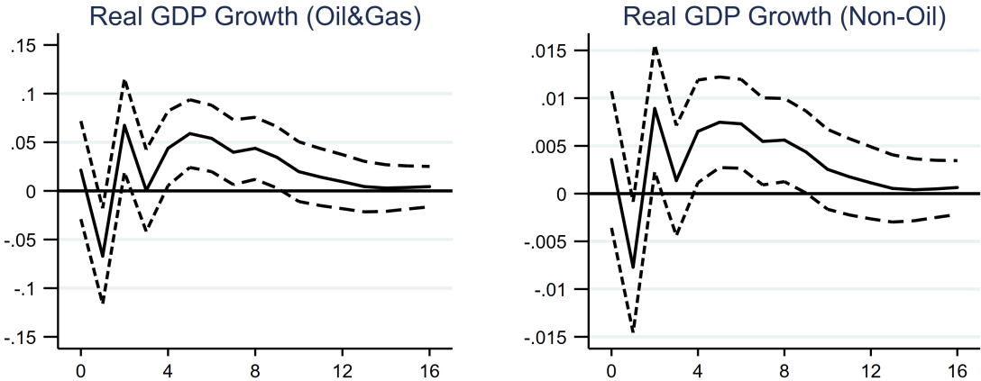
Figure 4: Dynamic Multipliers of Five-Variable VAR (Production)
