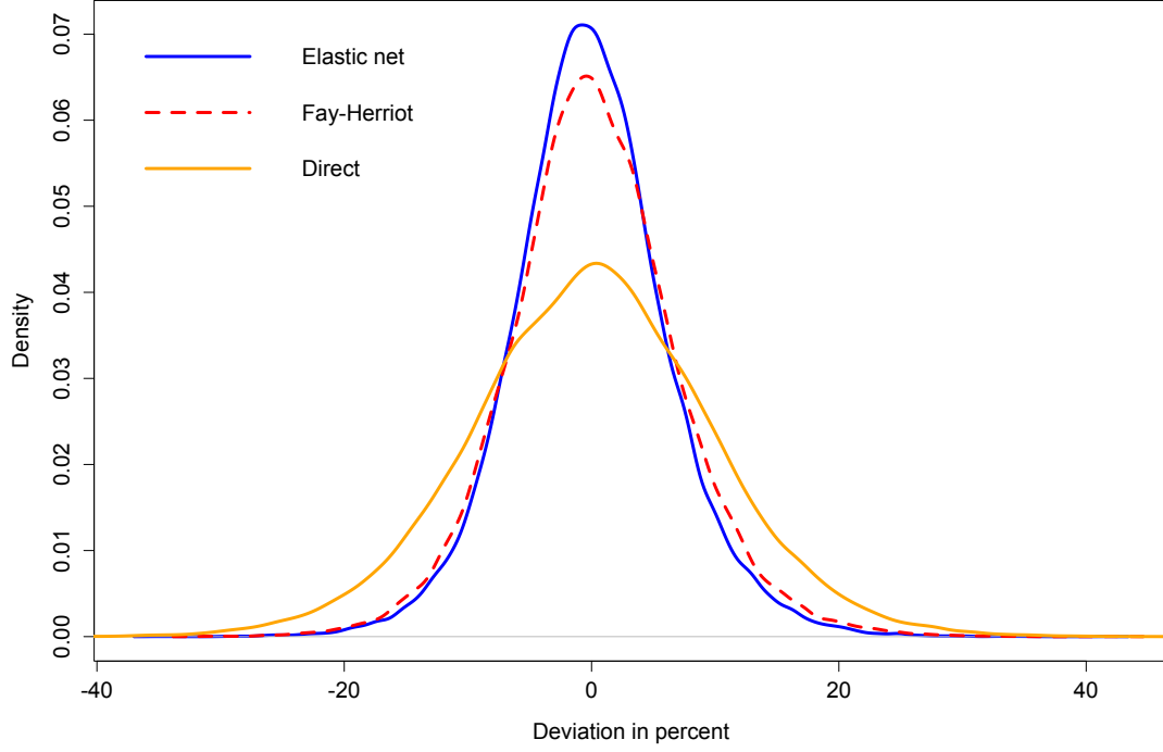
Figure 1: Distribution of the relative deviation, scenario 7
