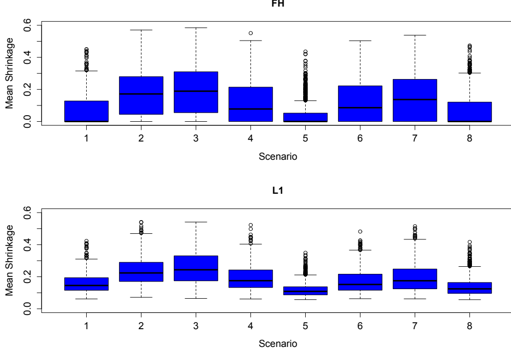
Figure 2: Distribution of the mean shrinkage factor over all areas
