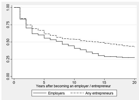
Figure 1: Kaplan-Meier survivor functions
