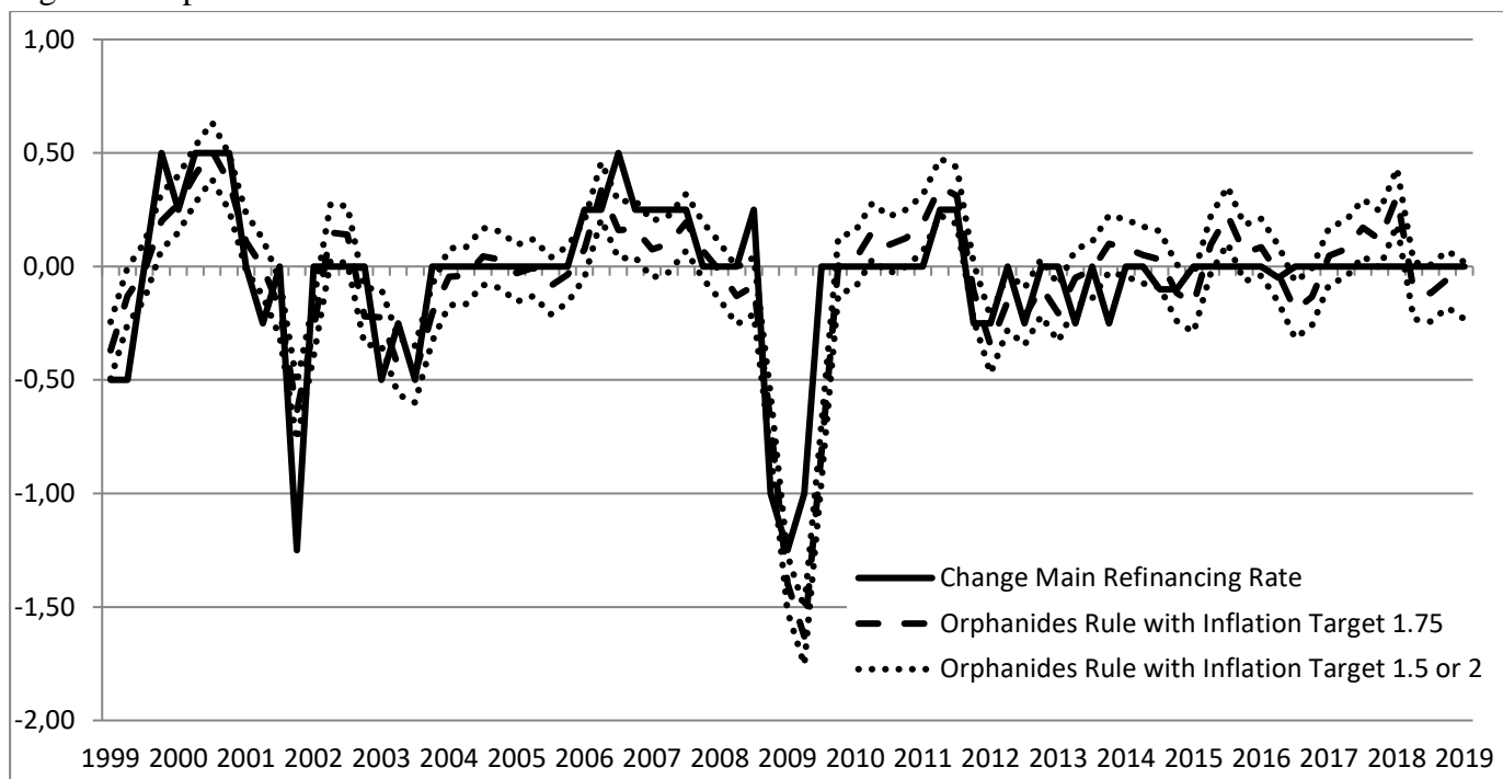
Figure 2: Orphanides-Rule
