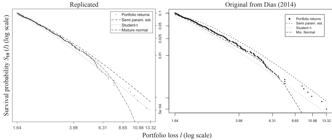
Figure 1: Loss survival probability plot of 10-asset portfolio
