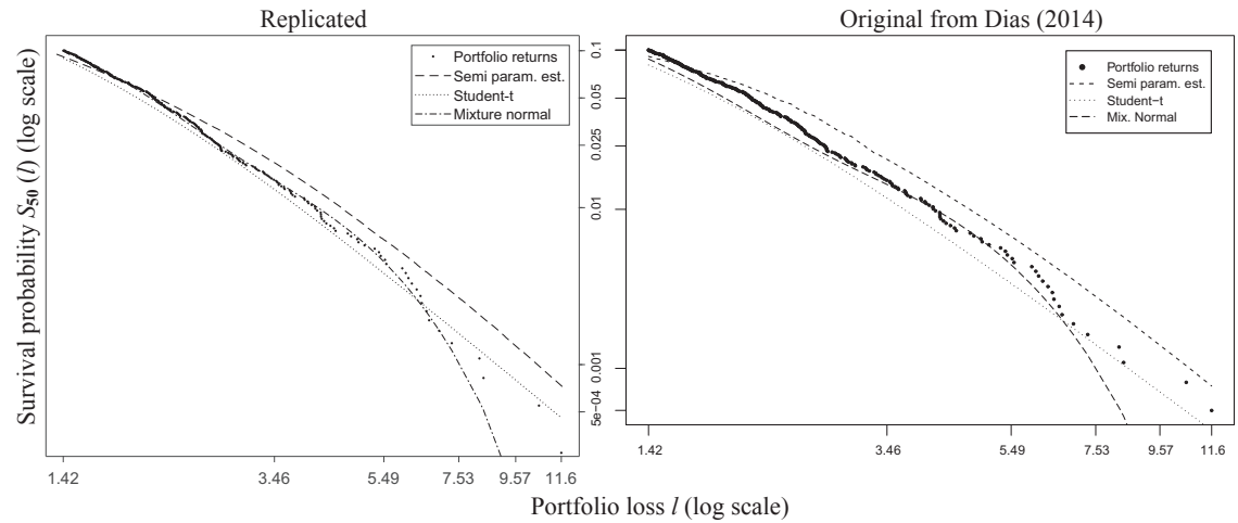
Figure 2: Loss survival probability plot of 50-asset portfolio
