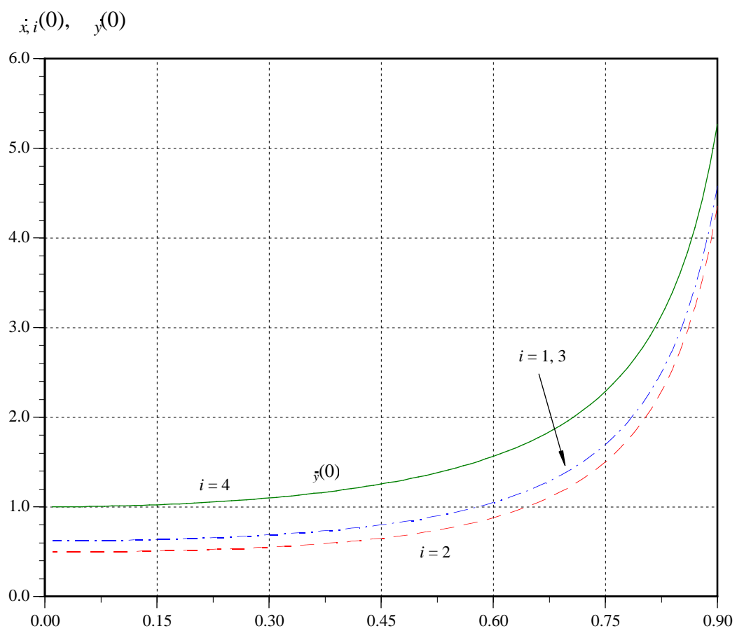
Fig. 1. Variance of the original series and periodic variances of the interpolated series evaluated at various \tau 's.
