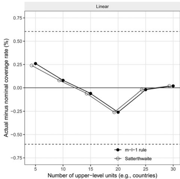
Figure 4. Performance of degrees of freedom approximations for the sampling distribution of test statistics in multilevel linear models Note: The figure shows percentage point deviations of actual coverage rates from the nominal value of 95 per cent. The horizontal zero line denotes the reference of accurate coverage (i.e., actual equals nominal coverage rate) based on 5,000 Monte Carlo replications. The dashed horizontal lines indicate 95 per cent test intervals that are constructed in the same way as in Figure 3. This figure has no correspondence in Stegmueller (2013).
