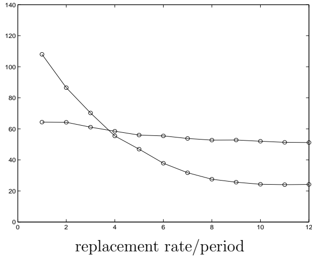
Figure 7: UI contracts
