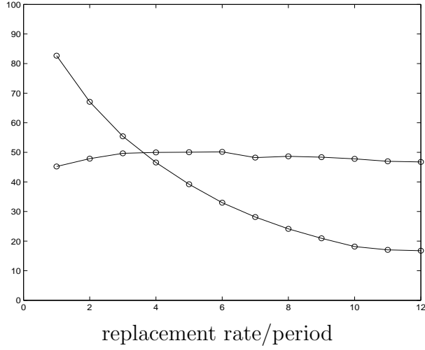
Figure 8: UI contracts
