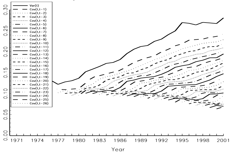
Figure 3: Variance-Covariances
