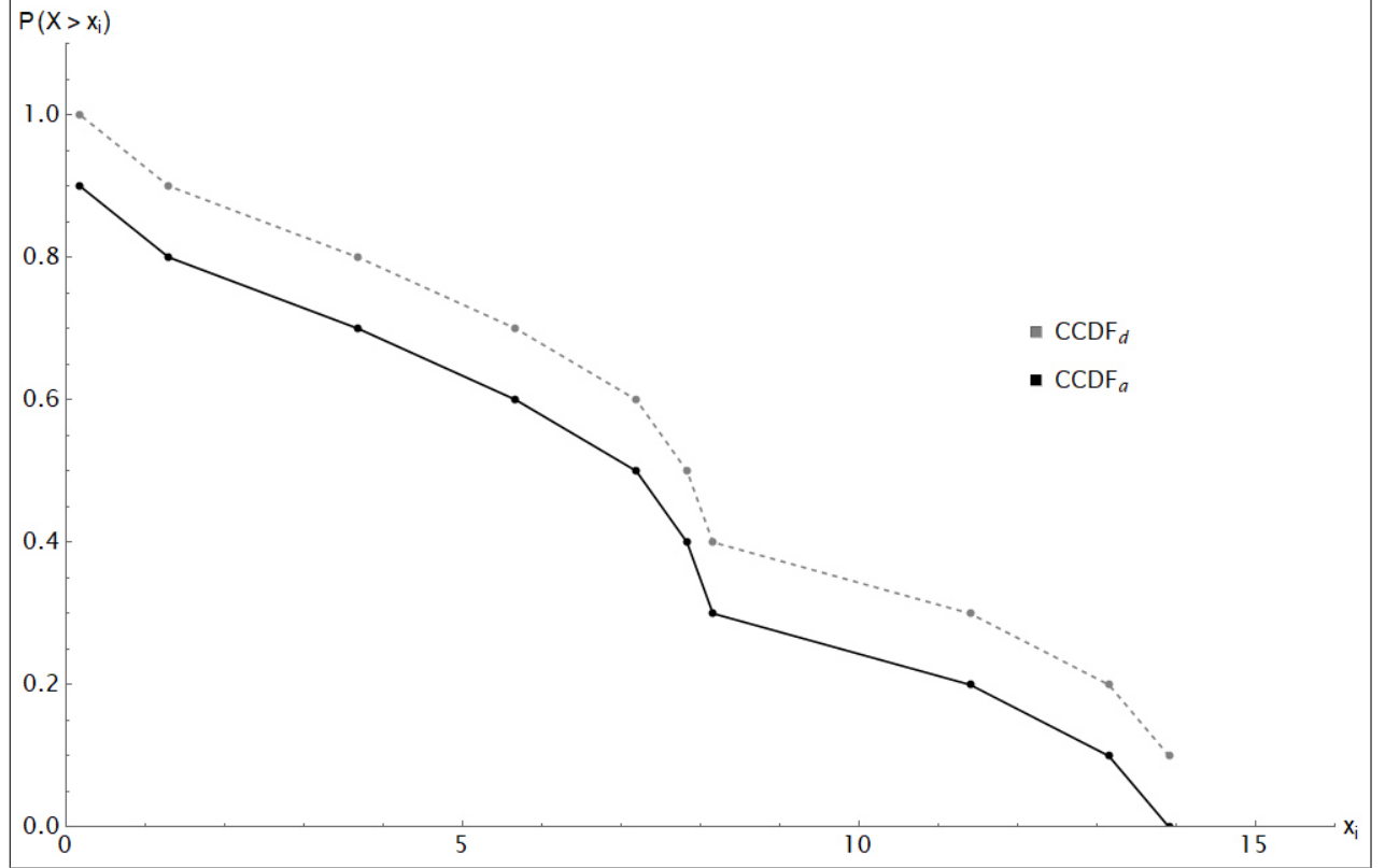
Figure 1: Different empirical CCDFs
