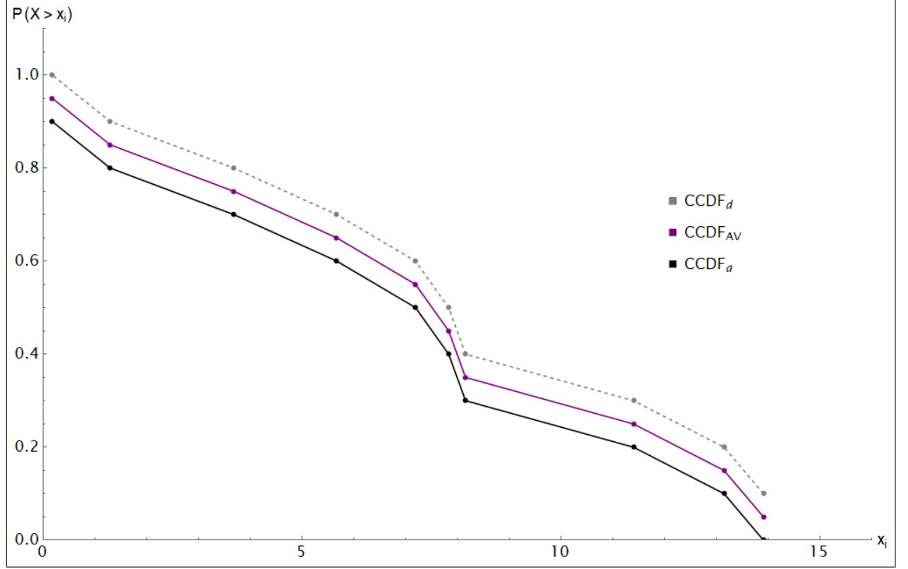
Figure 2: Different empirical CCDFs
