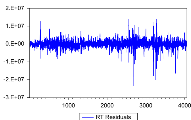
Figure 2. Residuals series of TUNINDEX Return during the period from 31 December 1997 to 07 April 2014.
