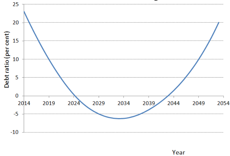
Figure 4: Debt Ratio Path in the Tax Smoothing Case
