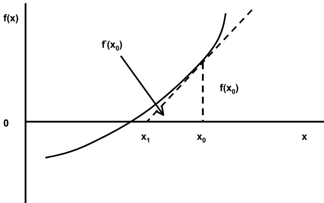
Figure 4 – Newton's method
