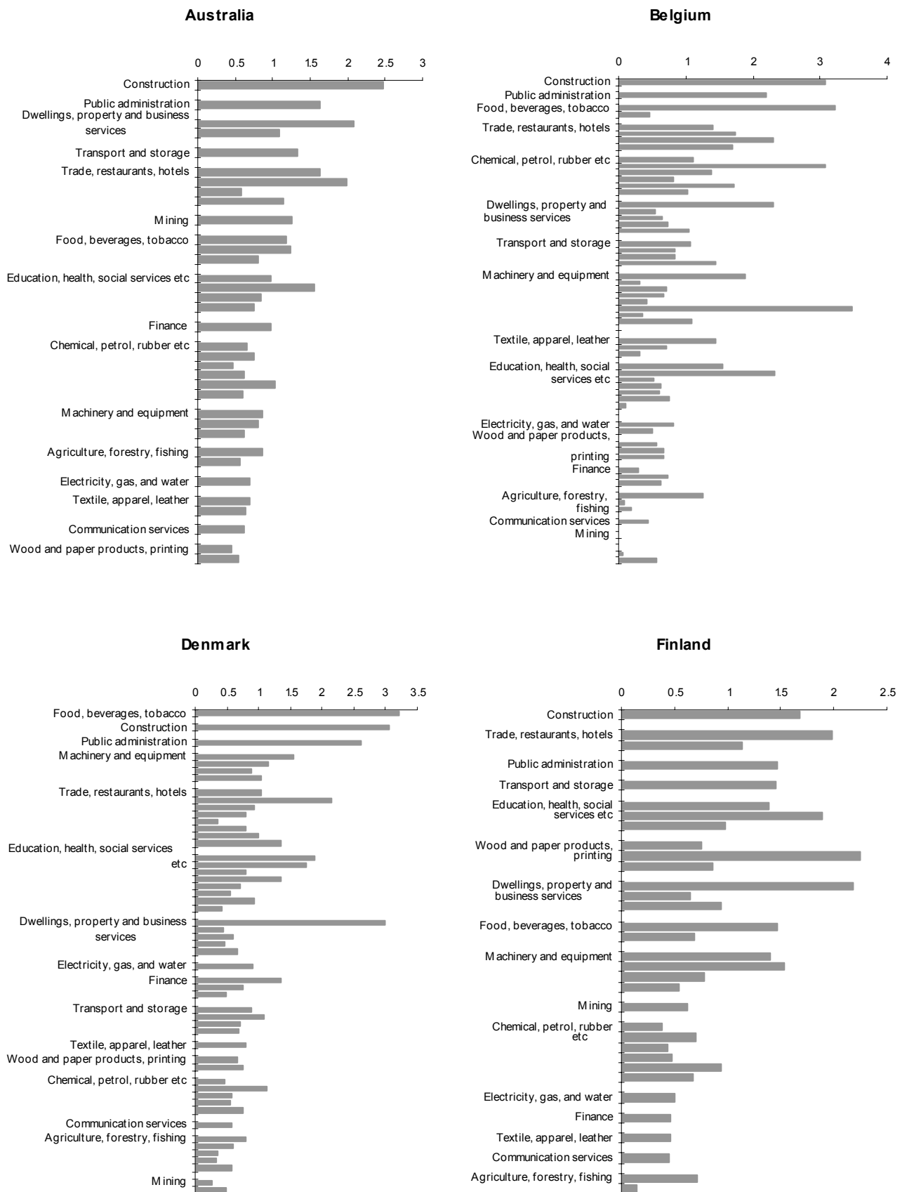
Figure 3: Backward linkages (final demand weighted) 15
