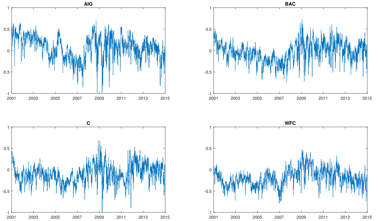
Figure 3: Fitted total daily log-volatilities
