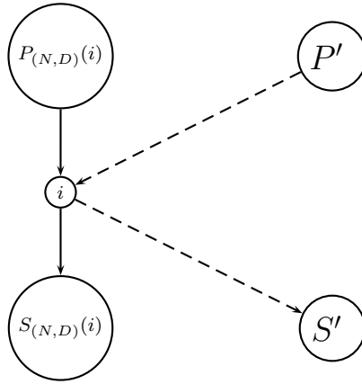
Fig. 6. Axiom 7 – entrance of a sybling of i if P_{(N,D)}(i) \cap S_{(N,D)}(i) = \emptyset , the dashed arrows represent the added arcs.
