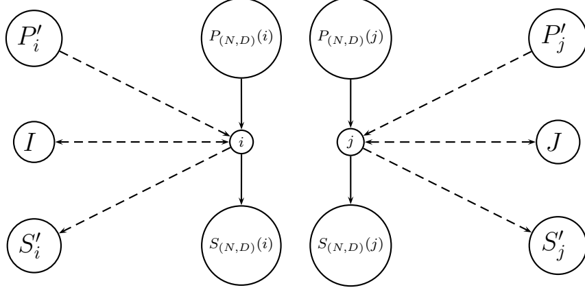
Fig. 7. Proof of Lemma 1 – Case A
