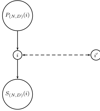
Fig. 3. Axiom 6 – entrance of a sybling of i if P_{(N,D)}(i) \cap S_{(N,D)}(i) = \emptyset , the dashed arrows represent the added arcs.
