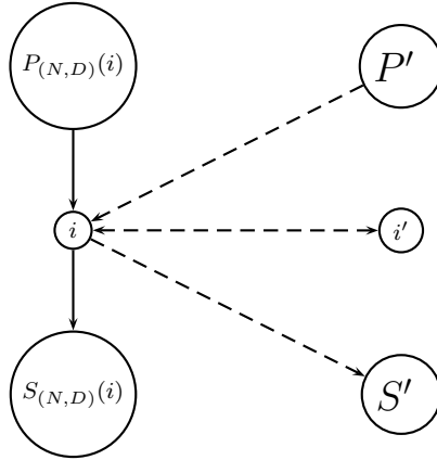
Fig. 2. Axiom 4 – entrance of a sybling of i if P_{(N,D)}(i) \cap S_{(N,D)}(i) = \emptyset , the dashed arrows represent the added arcs.
