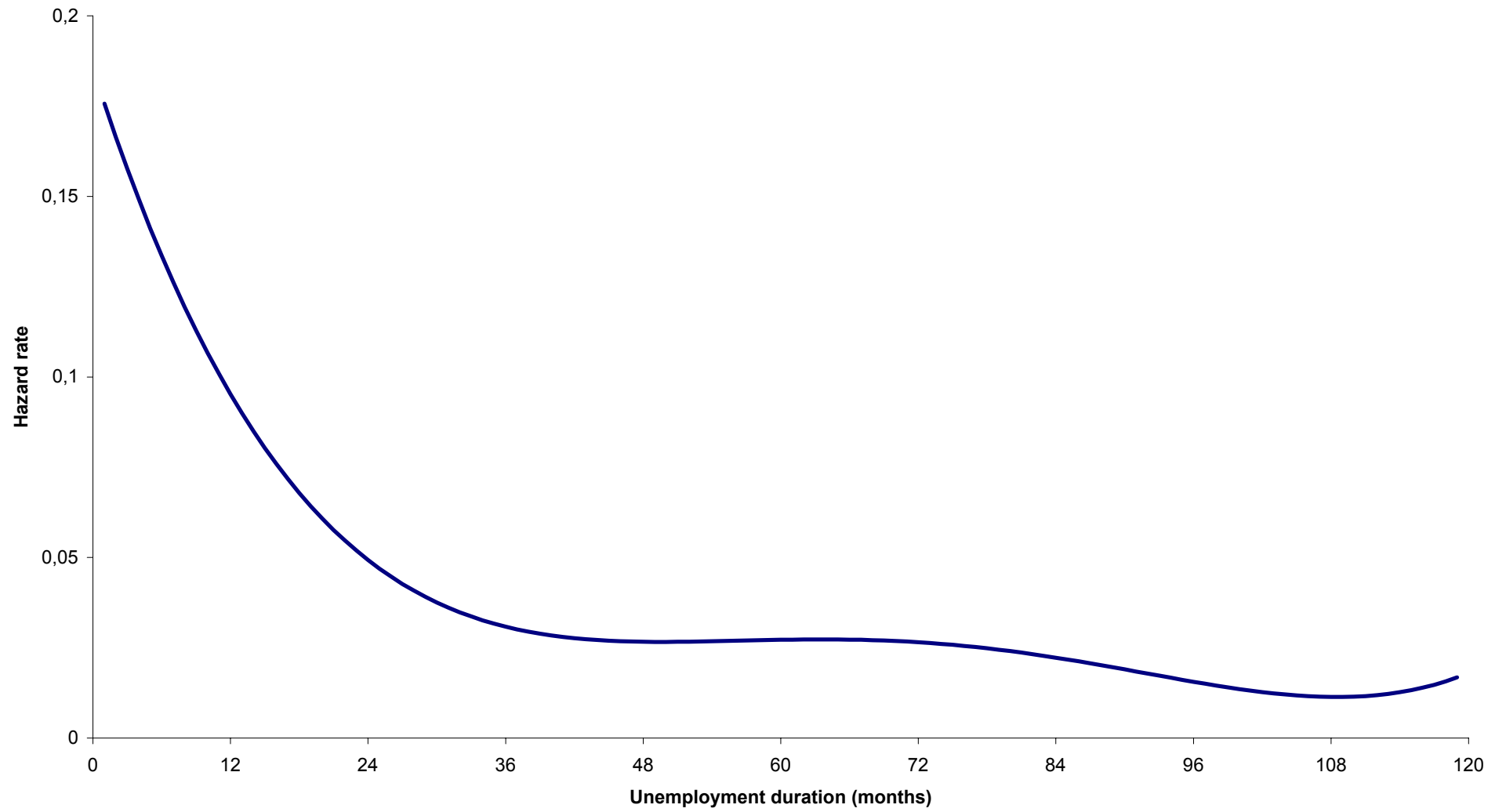
Figure 1: Baseline Hazard Function (4th degree polynomial function)
