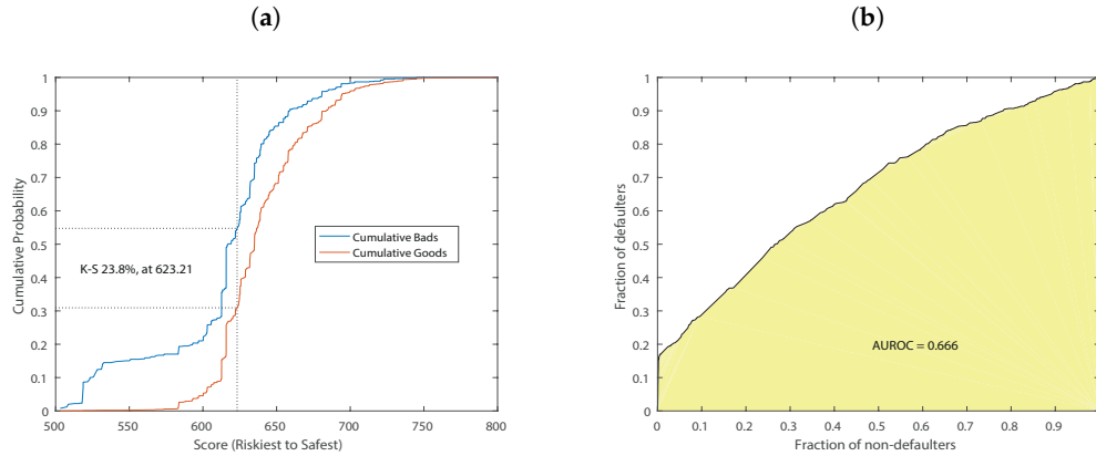
Figure 2: Panel (a) illustrates the Kolmogorov-Smirnov curve and the associated statistics for the first pool cut-off date. We show that the KS statistic associated to a score of 623.21 is 23.8%. Panel (b) reports the ROC curve and the AUROC value for the first report date. Table 6 reports AUROC, KS statistic and KS score for the entire sample.
