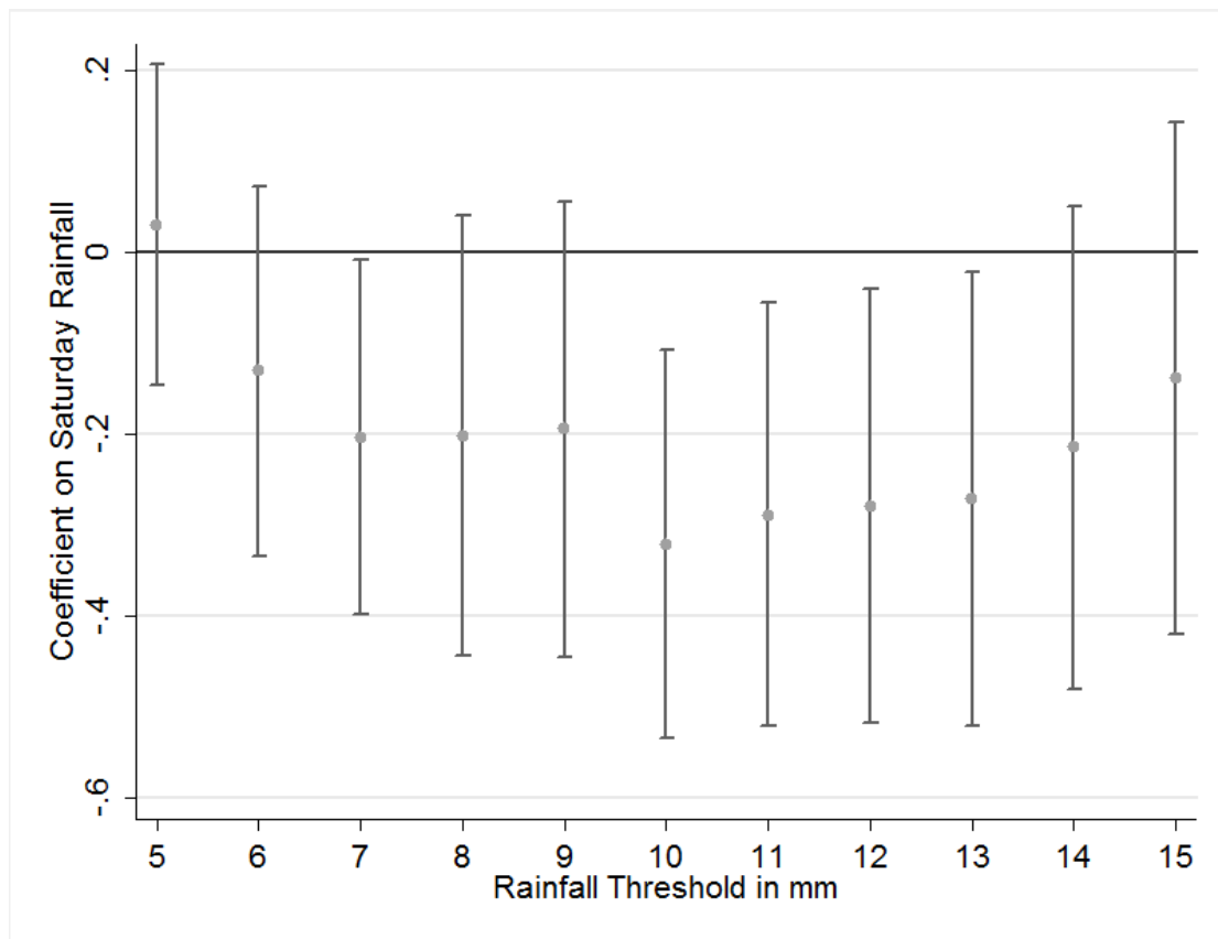
Figure 5: Different Thresholds
