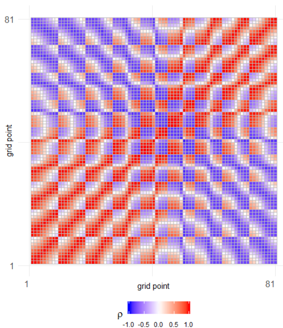
Figure 2: Correlation Matrix for N = 10,000 and R = 81
