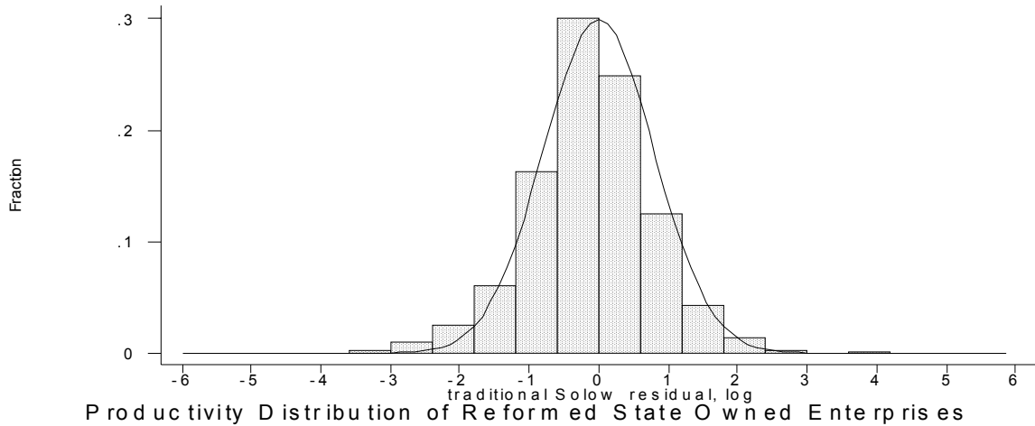
Figure 2: Reformed State Owned Enterprises Productivity Distributions from OLS, 2-Step & 3-Step procedures, respectively
