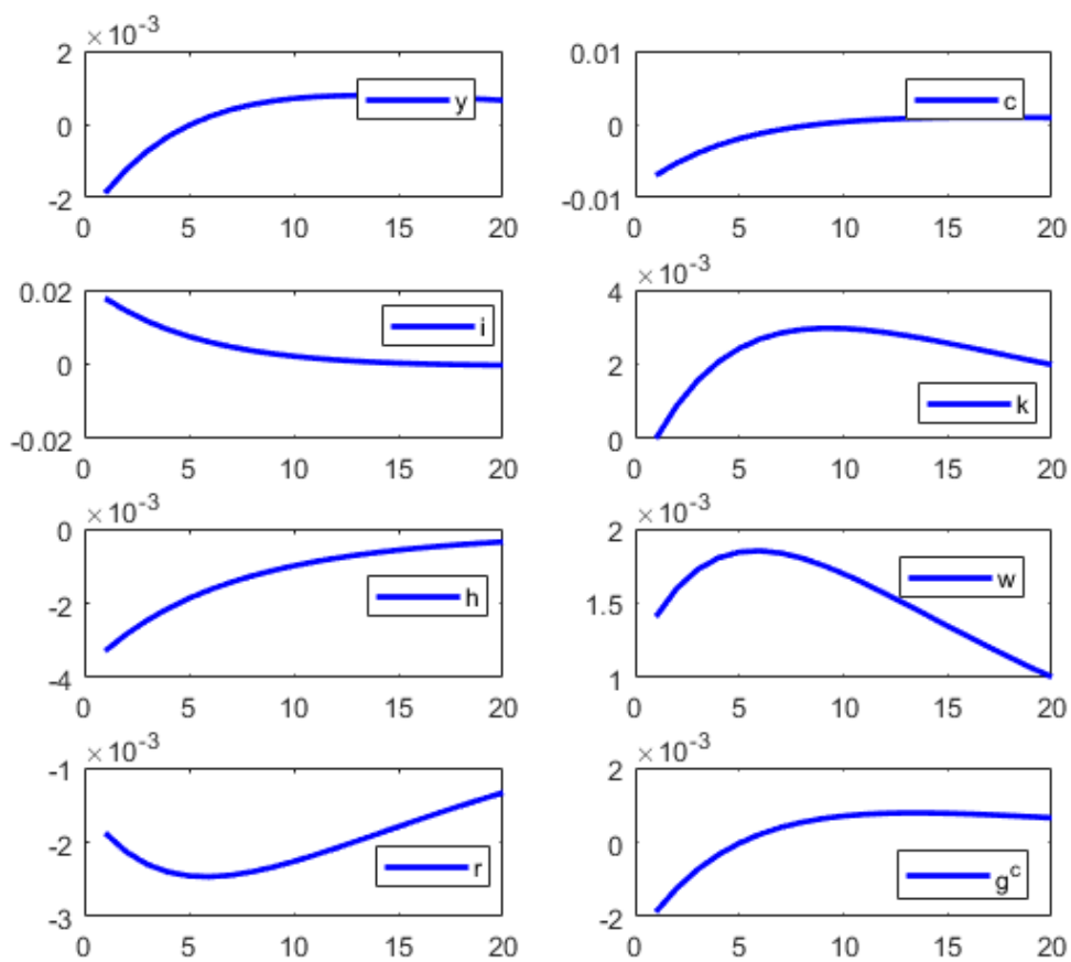
Figure 3: Impulse Responses to a 1% surprise innovation in consumption confidence
