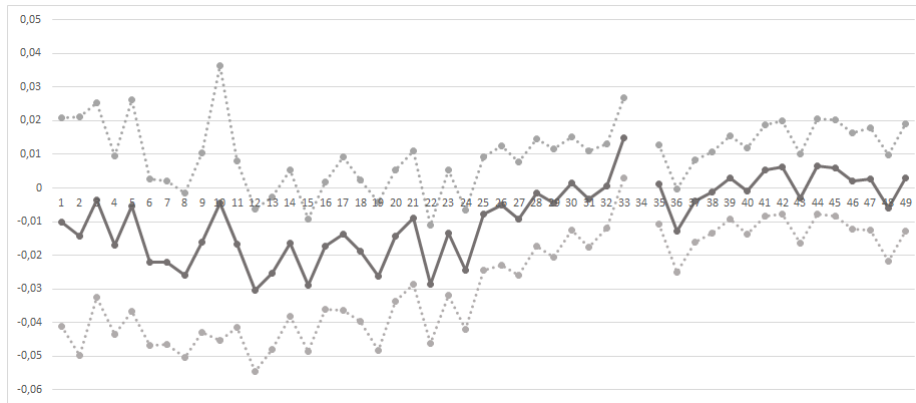
Figure 22: Event study log(view) (advertising YouTubers). The dark grey dots and the solid line represent the estimates \hat{\gamma}_t''' from equation (19). The dashed line depicts a 95%-confidence interval.
