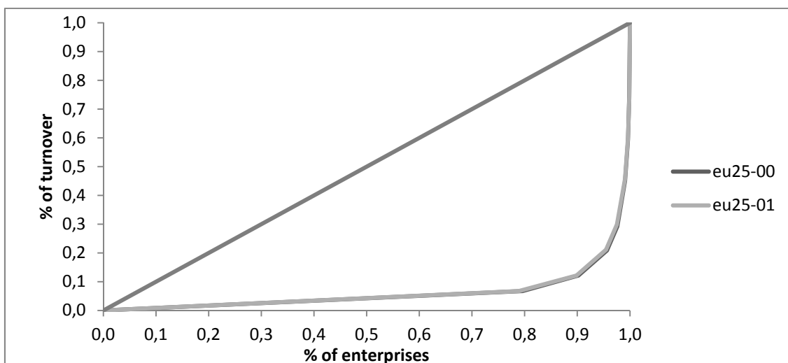
Figure 3: Lorenz curve 2000-2001
