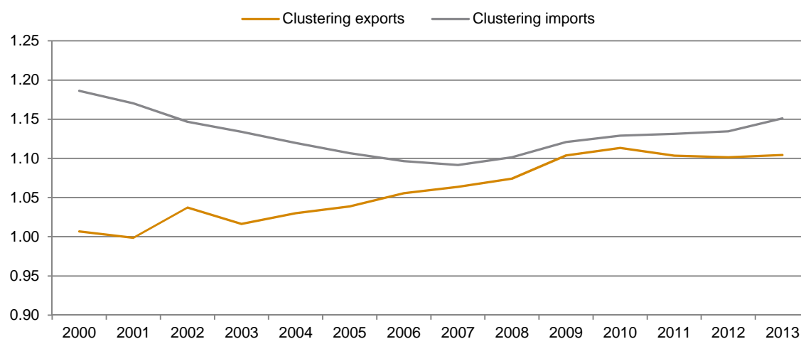
Figure 2.7.6 / Clustering measure
