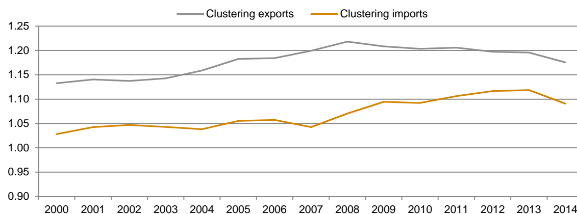
Figure 2.3.7 / Clustering measures
