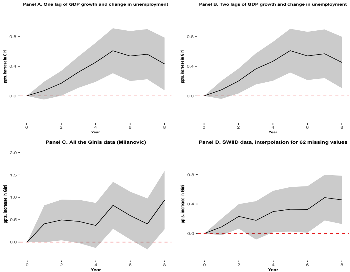
Figure 7: Robustness checks: Variations in Gini data
