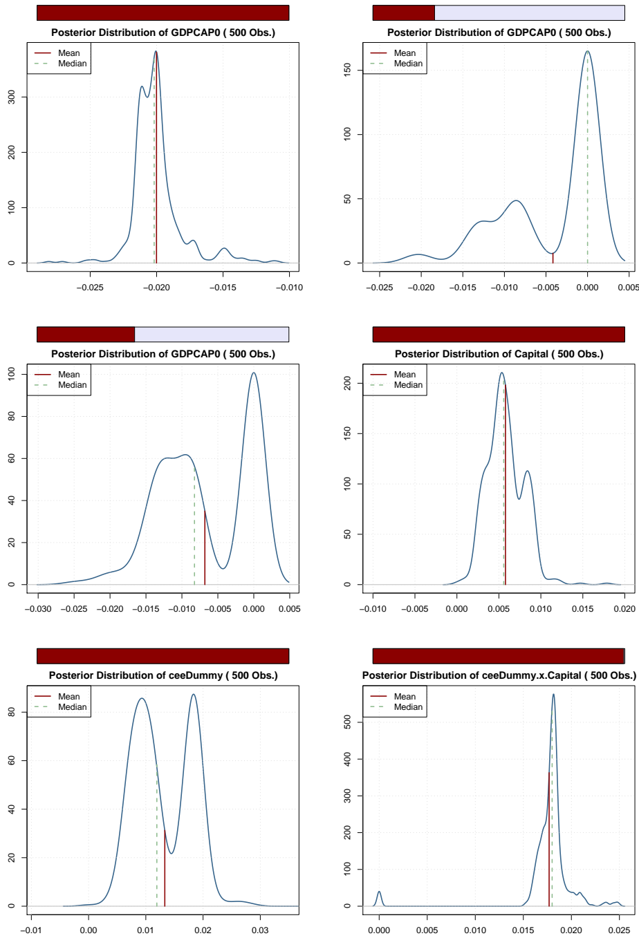
Figure 3: Unconditional posterior distribution (500 best models). Red bars on top of each distribution refer to the posterior inclusion probability of the respective regressor. Top panel, left side shows the posterior distribution of the initial income variable (GDP- CAP_0 ) based on the model specification not including the CEE dummy variable (Table 3, first column). Top panel, right side is based on the model including the CEE dummy variable (Table 3, second column). Middle and bottom panel are based on the estimation given in Table 3, third column. Distributions are shown for the initial income variable (GDP- CAP_0 ), the capital city dummy (Capital) and its linear interaction term (Capital \times CEE dummy).
