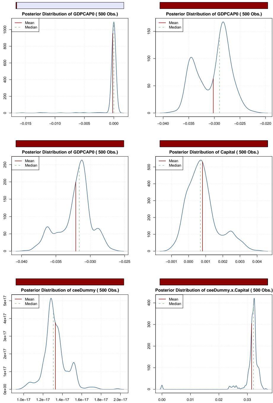
Figure 4: Unconditional posterior distribution based on models with fixed effects (500 best models). Red bars on top of each distribution refer to the posterior inclusion probability of the respective regressor. Top panel, left side shows the posterior distribution of the initial income variable (GDP0) based on the model specification not including the CEE dummy variable (Table 4, first column). Top panel, right side is based on the model including the CEE dummy variable (Table 4, second column). Middle and bottom panel are based on the estimation given in Table 4, third column. Distributions are shown for the initial income variable (GDP0), the capital city dummy (Capital) and its linear interaction term (Capital \times CEE dummy).
