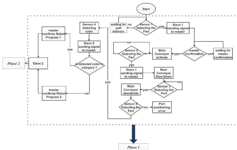
Figure 3. Main conveyor control architecture (phase 1).
