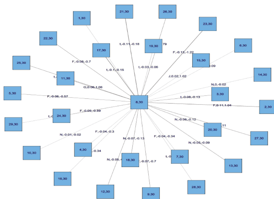
Figure 8. C-Vine Tree 2 Pre-GFC.
