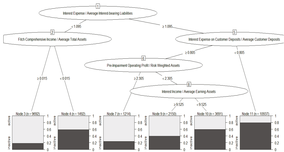
Figure 3. Plot of a tree model.
