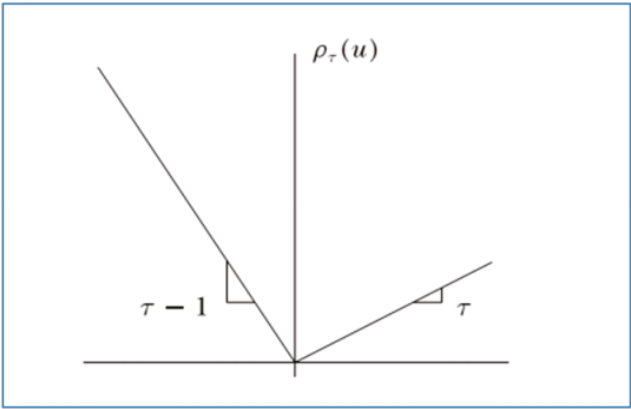
Figure 4. Quantile regression \rho function.
