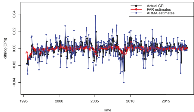
Figure 5. Estimated first order difference of the log-CPI given by the FAR(4,2) model and the ARMA(5,5) model.
