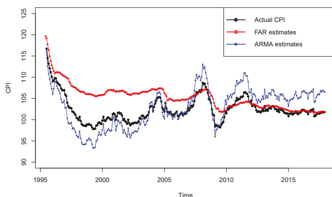
Figure 6. Estimated CPI given by the FAR(4,2) model and the ARMA(5,5) model.
