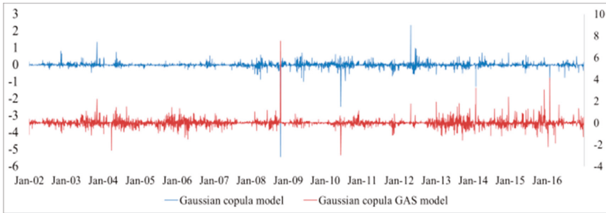
Figure 6. ΔCoVaR between Hungary and Germany. Note: This figure plots the estimated ΔCoVaR between Hungary and Germany from the Gaussian copula and Gaussian copula GAS models for 3-year yields (top), 5-year yields (middle), and 10-year yields (bottom) in the panel (A,B).
