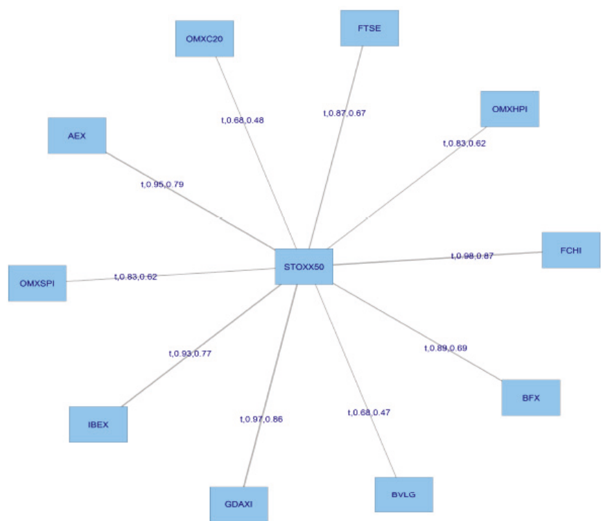
Figure 7. Results-C-Vine Tree-1 Pre-GFC.
