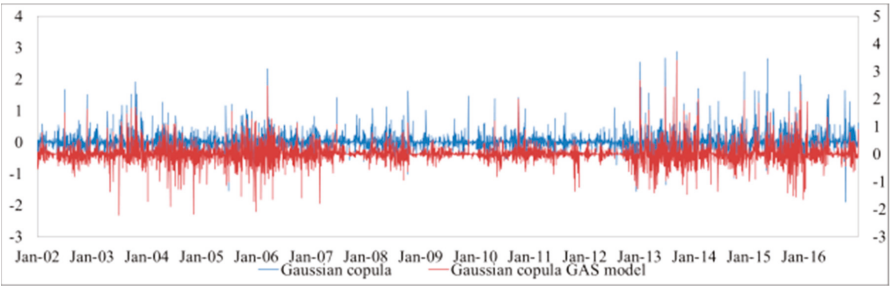
Figure 4. \Delta CoVaR between Poland and Germany. Notes: This figure plots the estimated \Delta CoVaR between Poland and Germany from the Gaussian copula and Gaussian copula GAS models for 3-year yields (top), 5-year yields (middle), and 10-year yields (bottom) in the panel (A,B).
