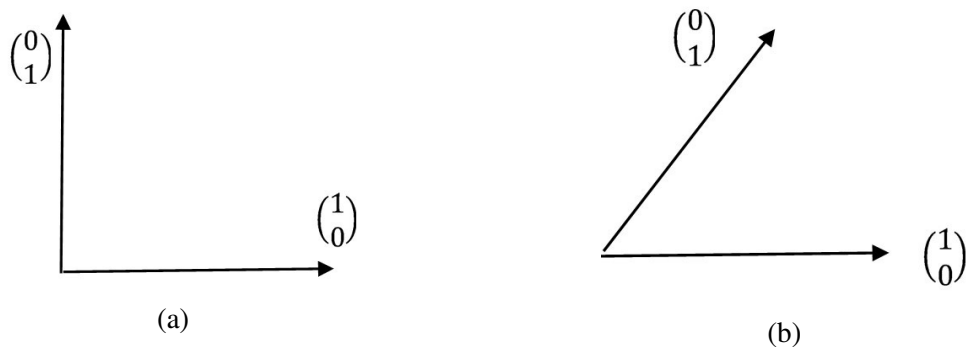
Figure 7: The axioms of vector spaces do not have a way to conceptualize if two vectors are orthogonal. The graphical difference between 7a and 7b does not have a mathematical counterpart yet.
