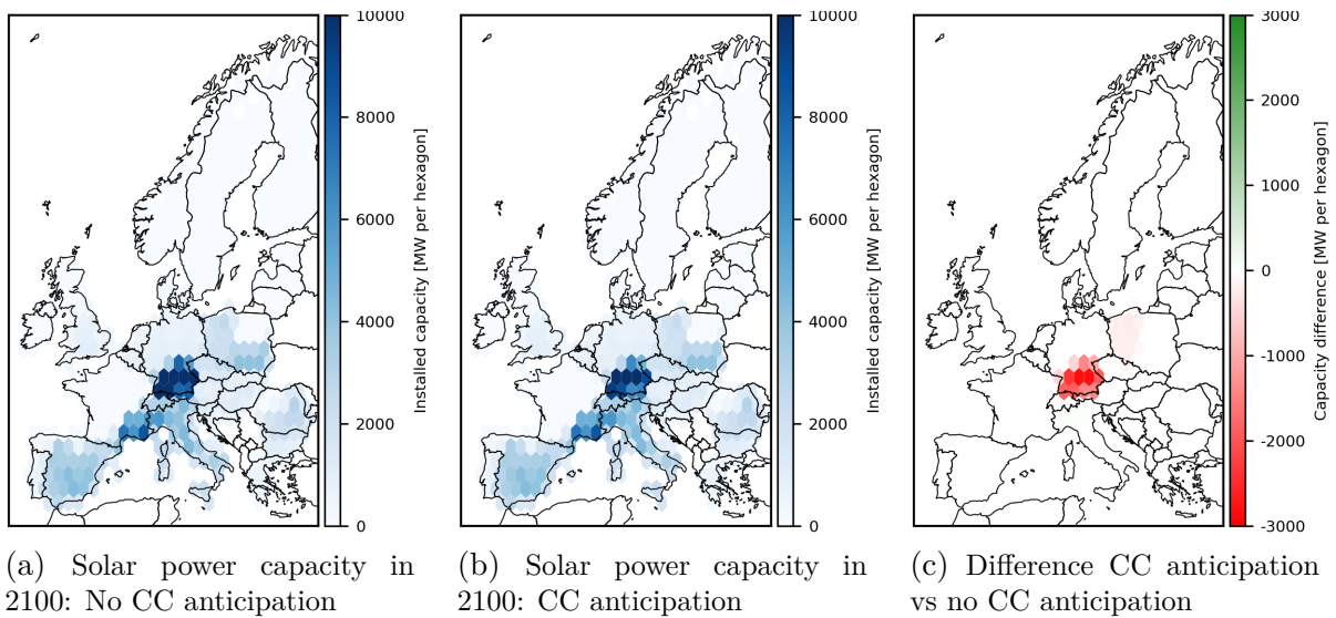
Figure 10: Allocation effects in optimal solar PV capacity of the CC-anticipation system compared to the No-CC-anticipation system in 2100.
