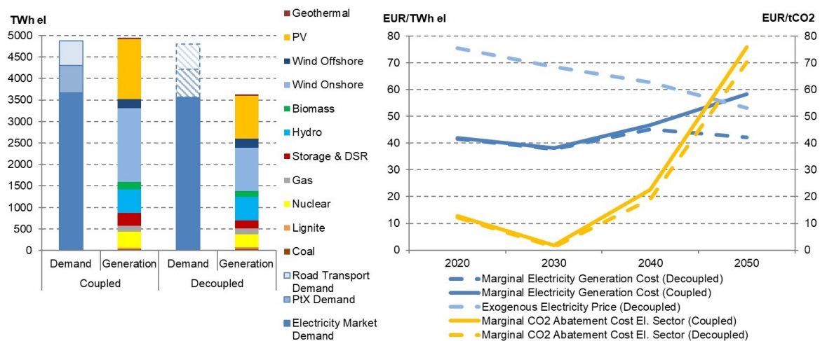
Figure 6: Electricity demand by module and electricity generation by fuel type in Europe in 2050 for the coupled and decoupled model (left); Results of average European marginal electricity generation costs and marginal CO 2 abatement costs for the electricity sector in the coupled and decoupled model, including the exogenous electricity price used by the decoupled road transport and energy transformation modules (right)
