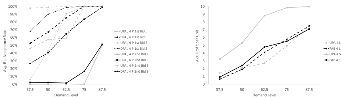
(a) avg. bid acceptance rates
