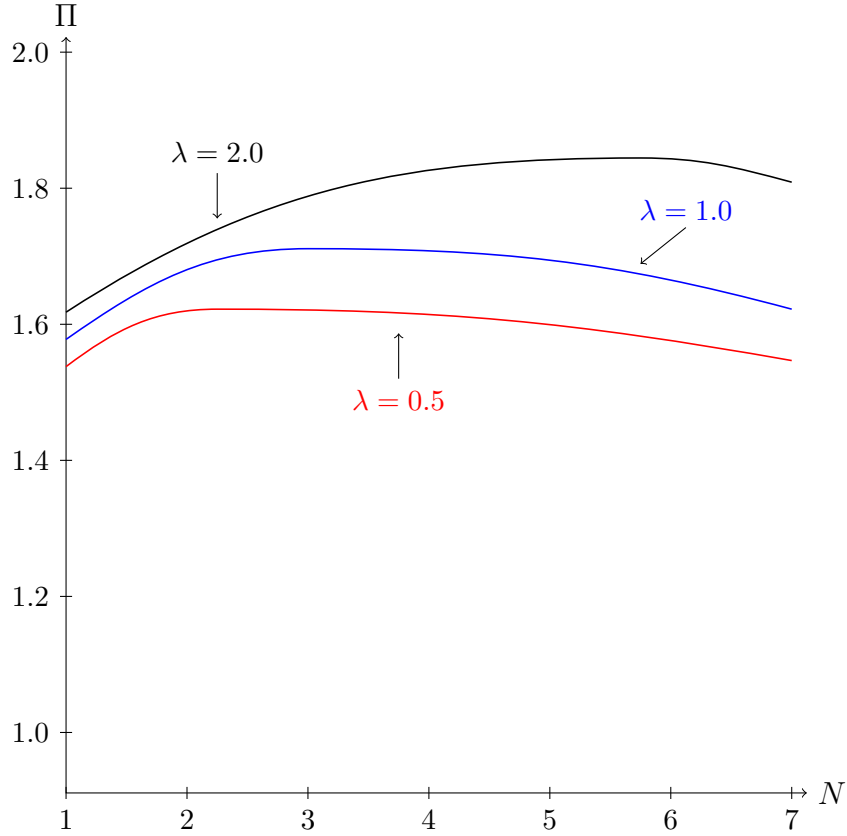
Figure 1: N^* for different values of \lambda
