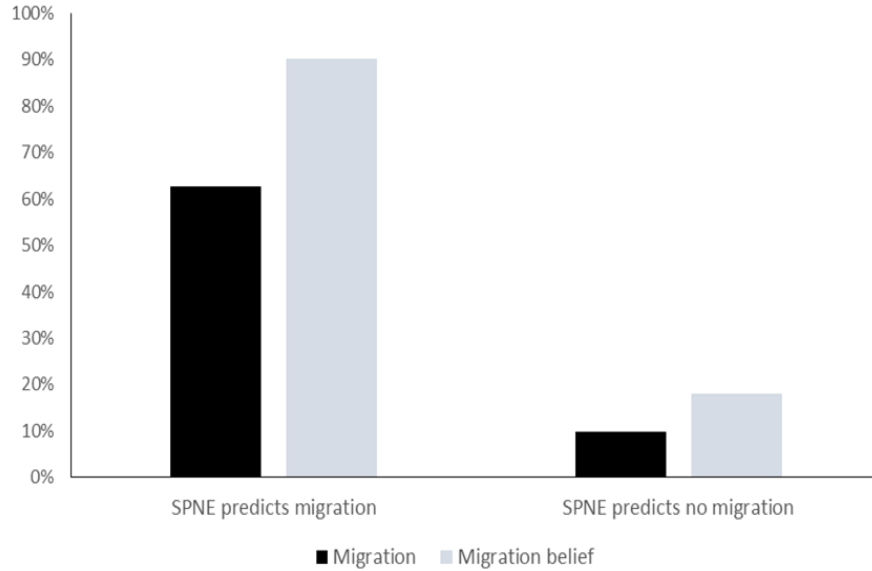
Figure 4: Migration choice and belief when SPNE predicts migration and otherwise
