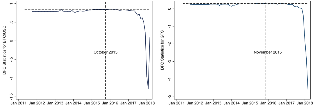
Figure 3: DFC Statistics for bubble detection in growth rates of BTC/USD and GTS
