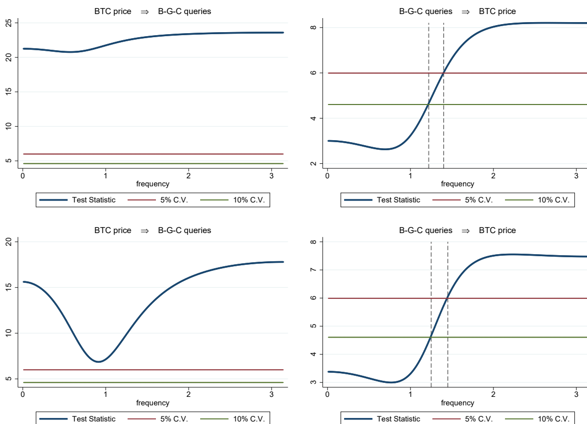
Figure 6: Spectral Granger causality tests using B-G-C queries as hype measure
