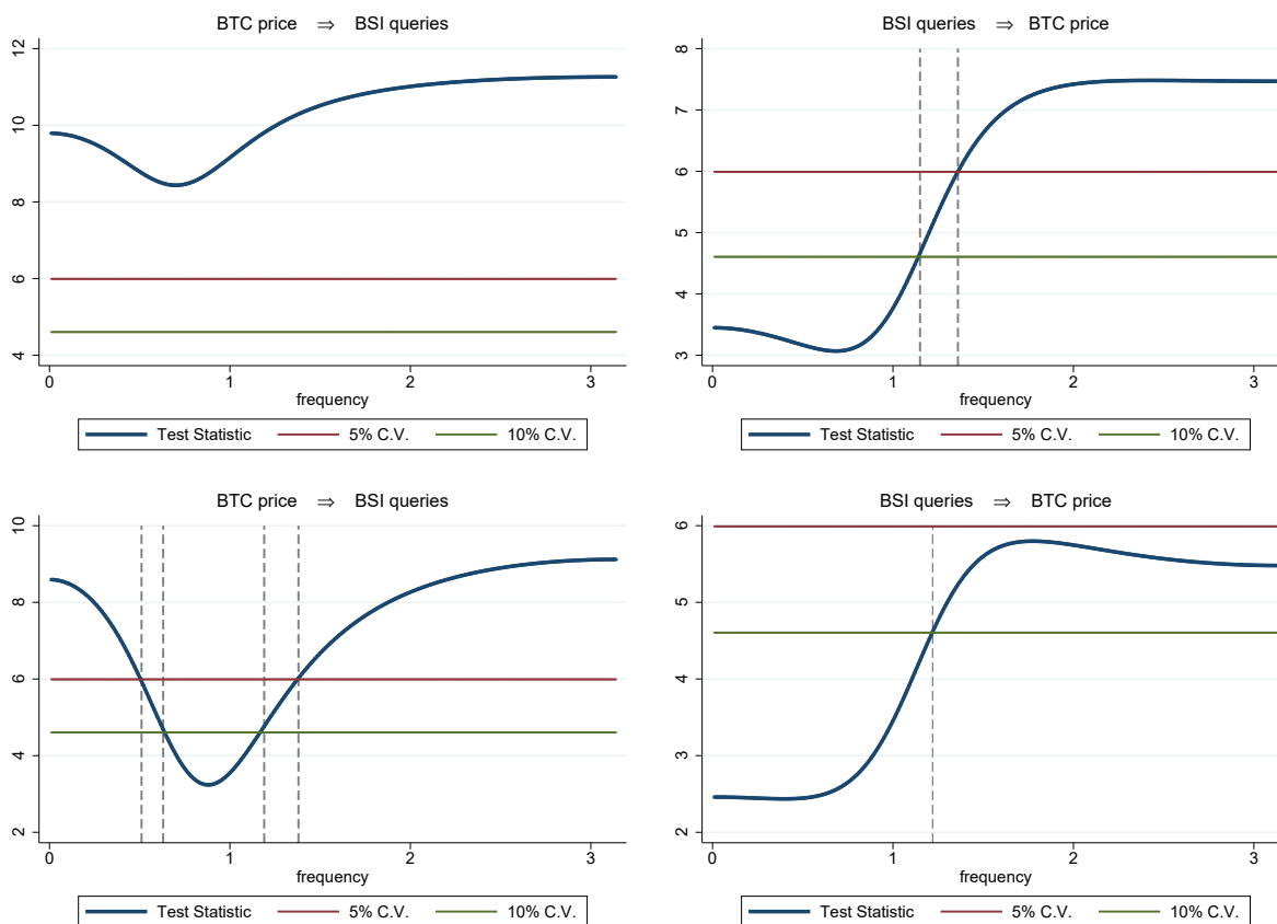
Figure 5: Spectral Granger causality tests using BSI queries as hype measure
