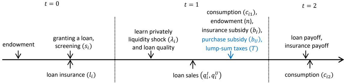
Figure 13: Timeline with subsidized purchases of uninsured loans.
