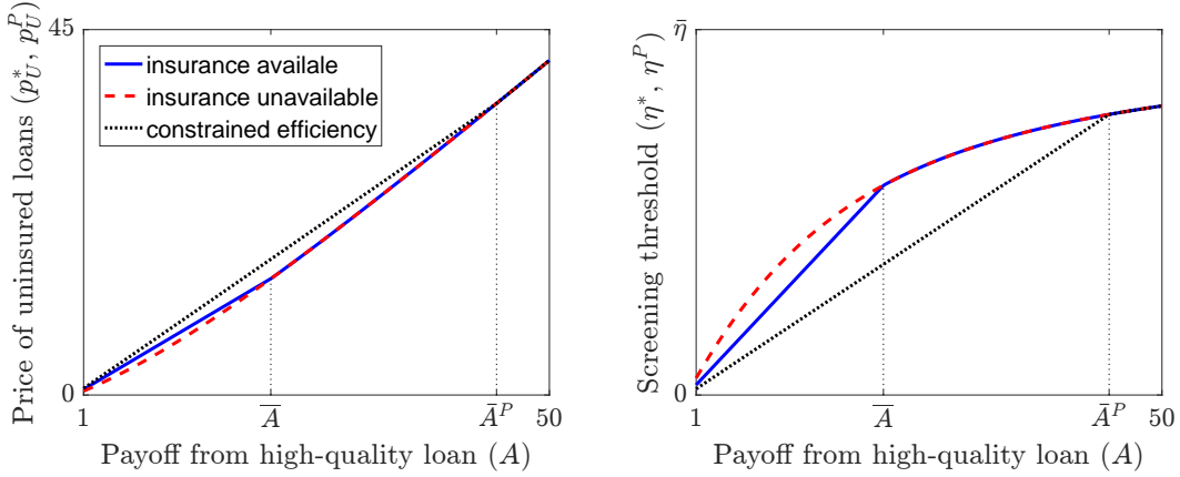
Figure 9: Constrained efficient levels of screening and prices of uninsured loans. Parameters: uniform distribution \eta_i \sim \mathcal{U} , \bar{\eta} = 1 , \nu = 0.1 , \lambda = 3 , \mu = 0.9 .
