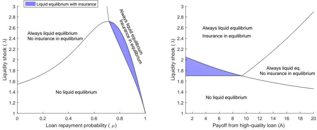
Figure 5: Existence of liquid equilibrium with loan insurance.
