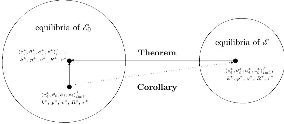
Figure 1: Corollary 3
