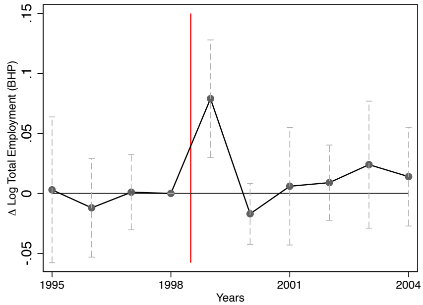
Figure 9: Dynamic Effect of Policy Change on Firm Employment Growth
