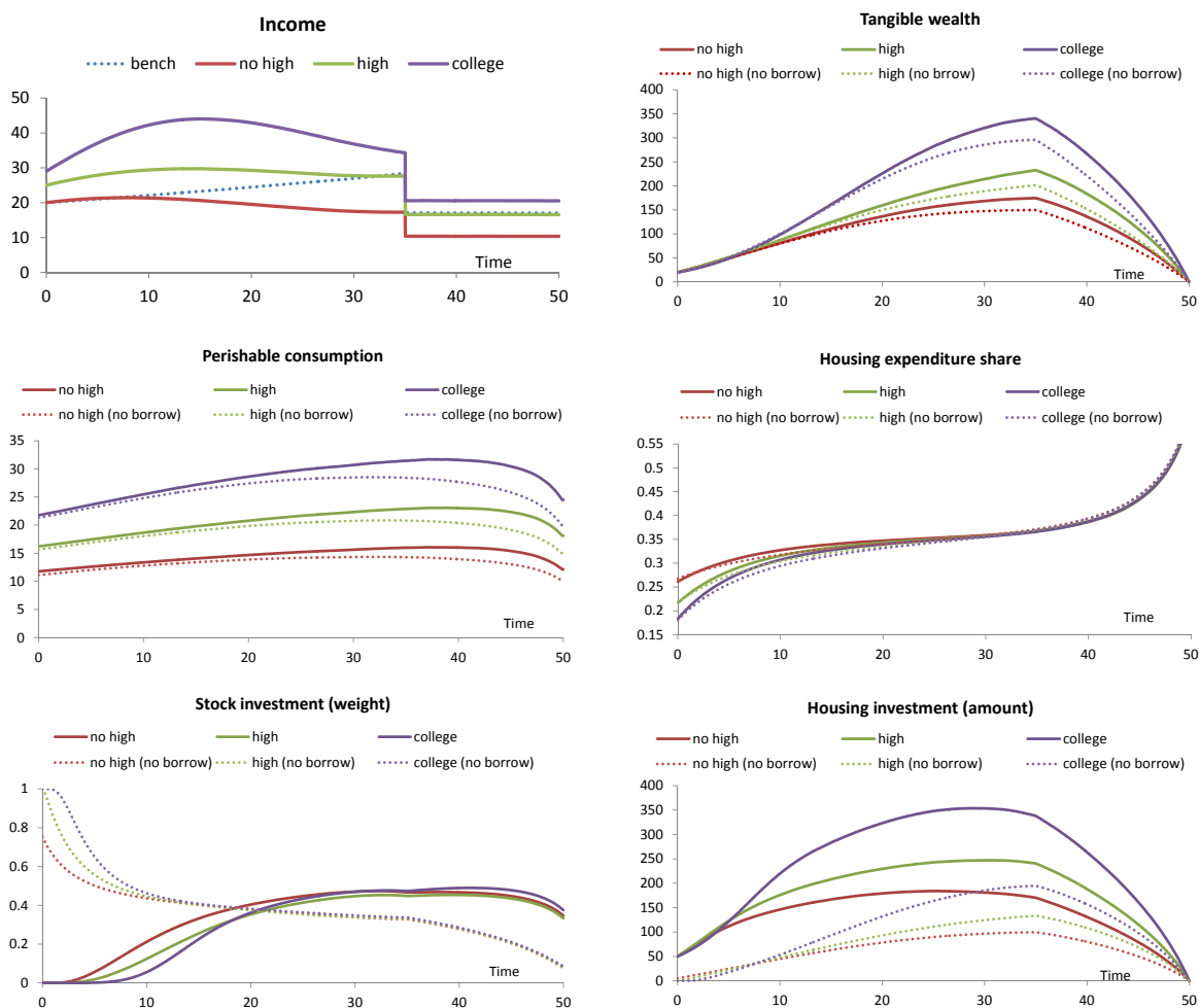
Figure 15: Consumption and investments for different educational levels. The average income profiles estimated by Cocco, Gomes, and Maenhout (2005) for three different educational groups are used. The solid curves are for the baseline case of \kappa = 0.4 (60% borrowing of house value), whereas the dotted curves are for the case \kappa = 1 (no borrowing). For all other parameters the baseline values in Table 1 are used.
