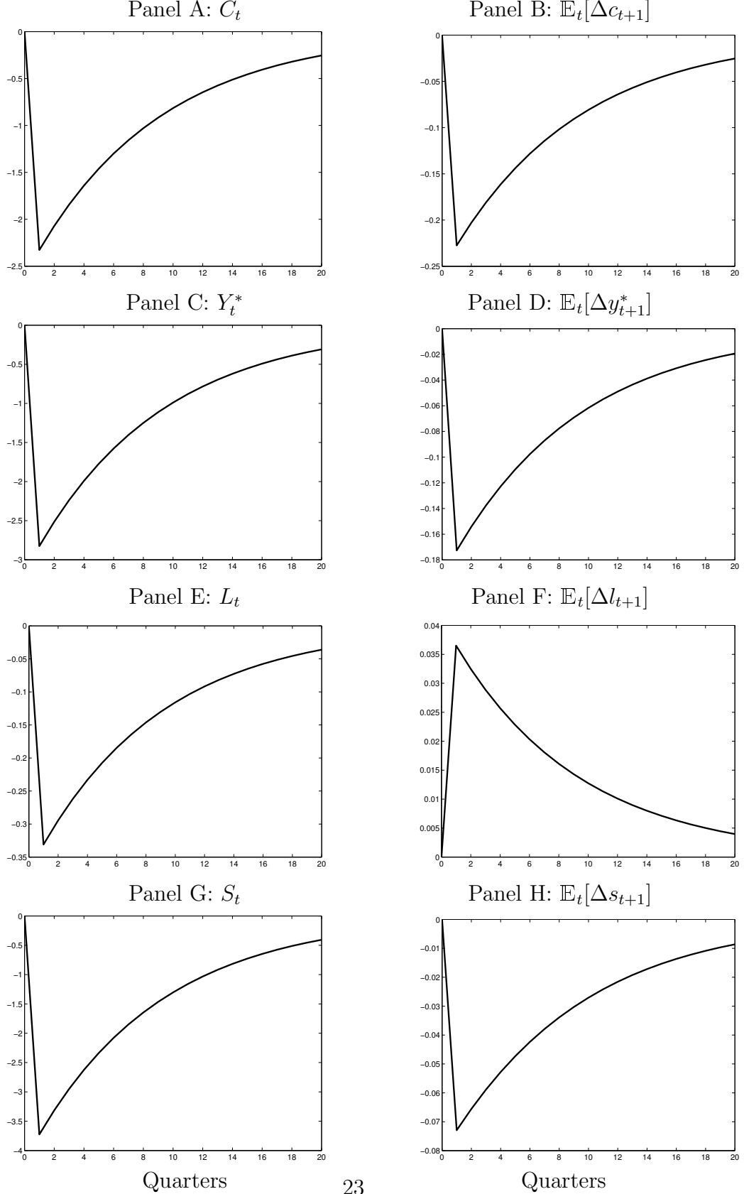
Figure 4: THE EFFECTS OF A NEGATIVE PRODUCTIVITY SHOCK. Notes: This figure depicts impulse response functions of consumption, C_t , expected consumption growth, \mathbb{E}_t[\Delta c_{t+1}] , total output, Y_t^* , expected total output growth, \mathbb{E}_t[\Delta y_{t+1}^*] , labor hours, L_t , expected labor hours growth, \mathbb{E}_t[\Delta l_{t+1}] , R&D expenditure, S_t , and R&D expenditure growth, \mathbb{E}_t[\Delta s_{t+1}] with respect to a negative one standard deviation shock to TFP, \Lambda_t ( \varepsilon_t^\Lambda ). Panels A, C, E, and G show log-deviations from the steady state in %, Panels B, D, F, and H show deviations from the steady state in %. Parameters are set as in Table 2.
